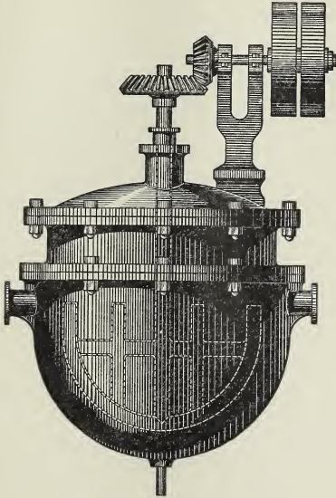
FIG. 11 b .—Zemsch's Varnish-kettle.
